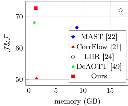
Fig. 4: Comparison of video object segmentation methods in terms of segmentation accuracy ( \mathcal{J}\&\mathcal{F} ) and memory footprint on DAVIS-17 Val dataset.
