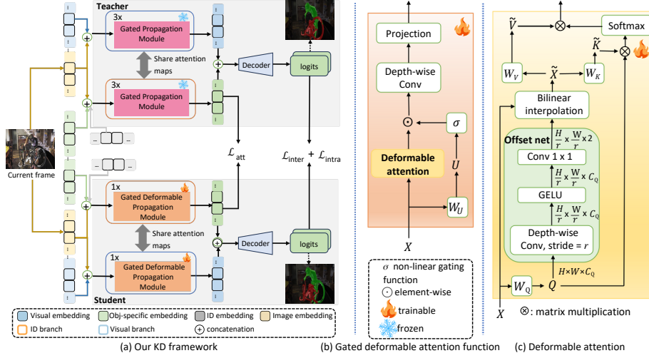
Fig. 2: Summary of our proposed VOS method. (a) Overview of our knowledge distillation method. The teacher model transfers intermediate attention maps to the student model. This transfer is enforced by a CKA-based loss \mathcal{L}_{att} . At the same time, probability distributions of logits are transferred using intra-object and inter-object losses \mathcal{L}_{intra} and \mathcal{L}_{inter} . Both the teacher and student models make use of Gated Propagation Module (GPM) [49], aiming to propagate spatio-temporal information across frames via the attention mechanism. (b) Our proposed Gated Deformable Attention function, which is used to implement the GPM. (c) Deformable attention module, which is used to replace the vanilla attention in the Gated deformable attention function.
