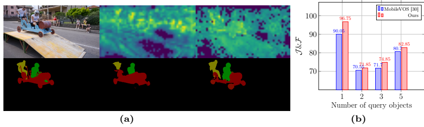
Fig. 1: (a) From left to right: input frame and ground-truth segmentation masks, distilled feature map and segmentation masks by the distillation strategy used in MobileVOS [30], distilled feature map and segmentation masks by our method. (b) Segmentation accuracy ( \mathcal{J}\&\mathcal{F} ) of MobileVOS [30] and our method with different numbers of query objects in DAVIS-17 val (see more details in Section 4).
